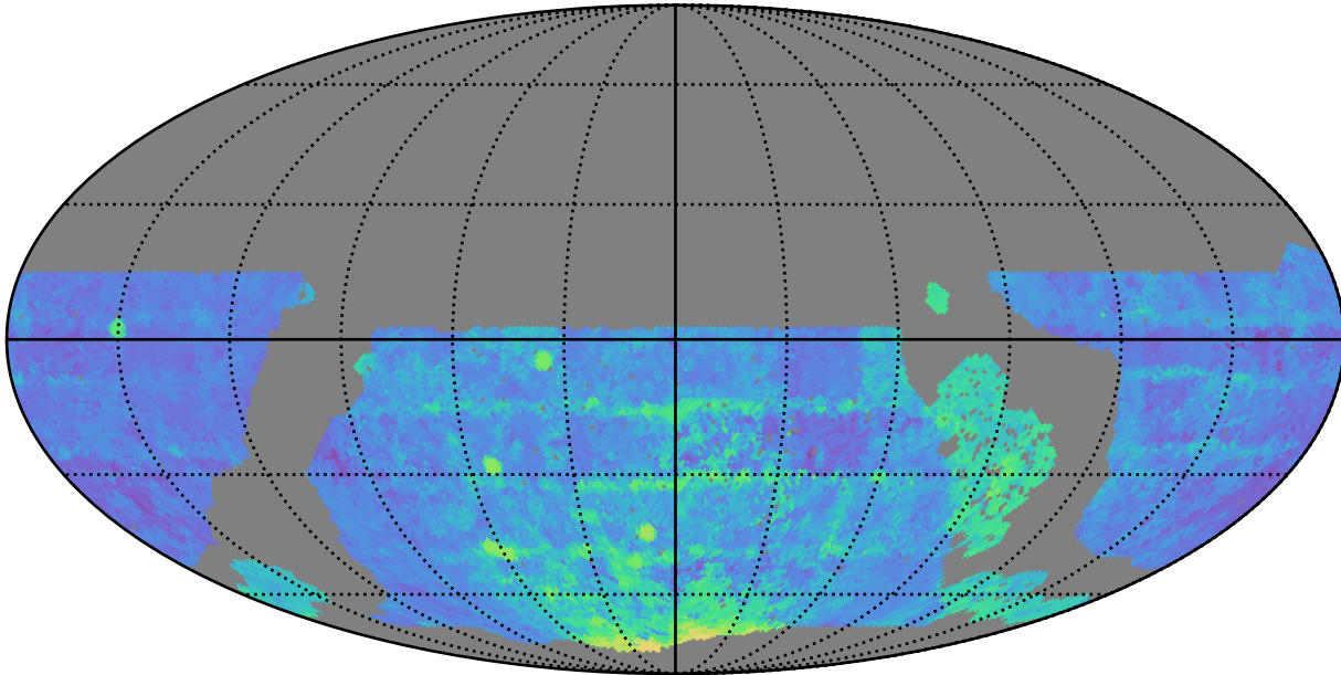
roll_uniform_early_half_accordion1_mjdp0_v3.4_10yrs WFD z band: Median Season Length
