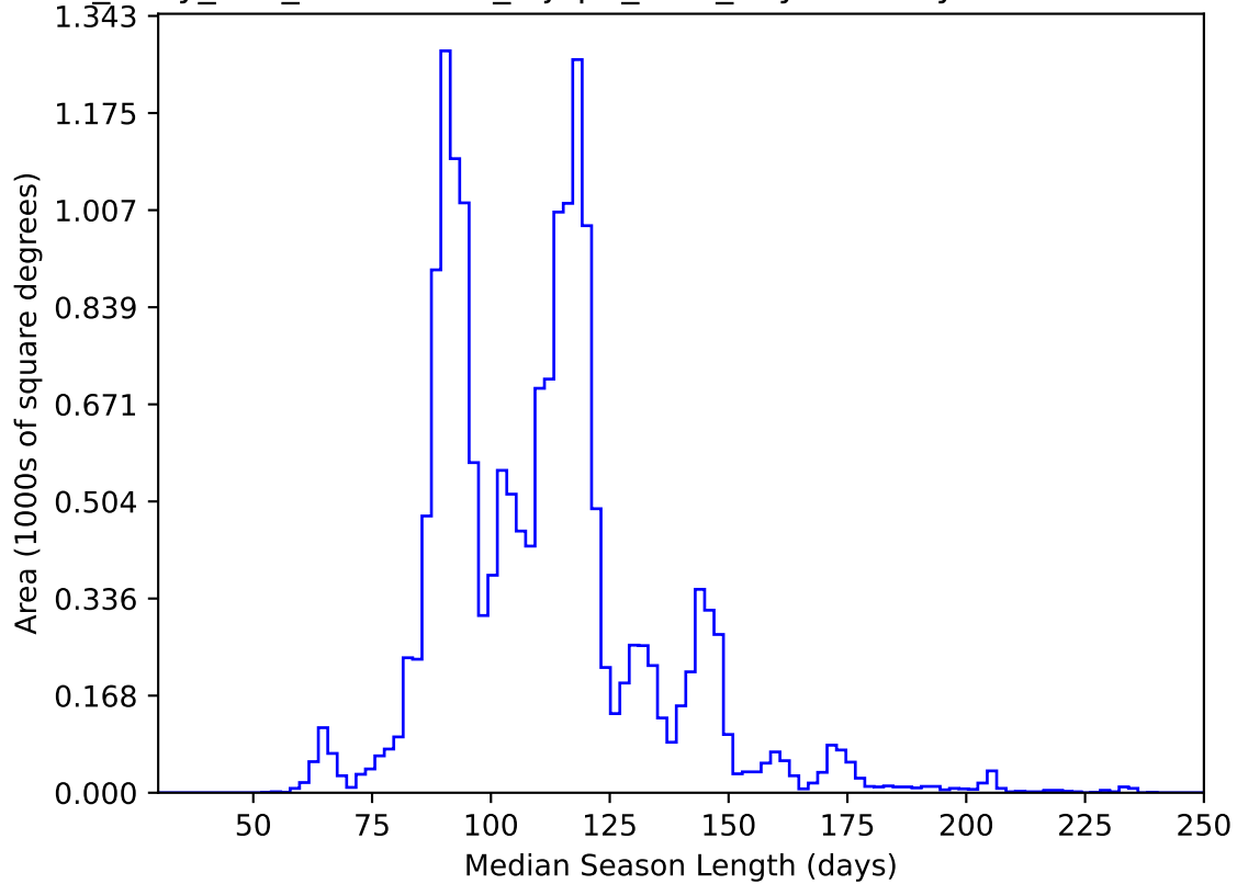
roll_uniform_early_half_accordion1_mjdp0_v3.4_10yrs WFD y band: Median Season Length
