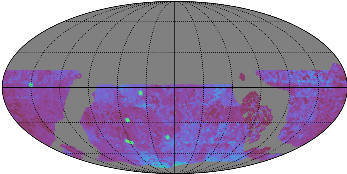
roll_uniform_early_half_accordion1_mjdp0_v3.4_10yrs WFD u band: Median Season Length
