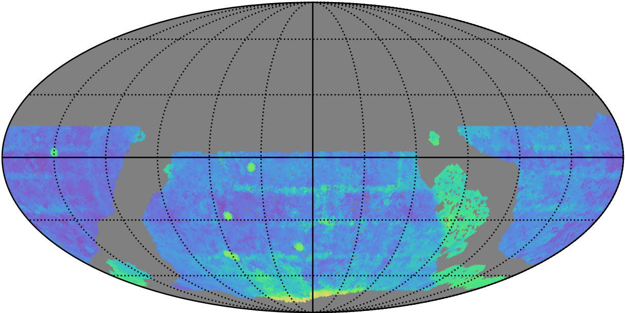
roll_uniform_early_half_accordion1_mjdp0_v3.4_10yrs WFD r band: Median Season Length
