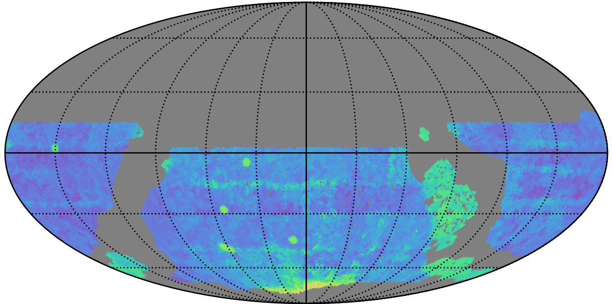
roll_uniform_early_half_accordion1_mjdp0_v3.4_10yrs WFD i band: Median Season Length
