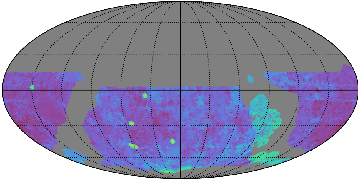
roll_uniform_early_half_accordion1_mjdp0_v3.4_10yrs WFD g band: Median Season Length
