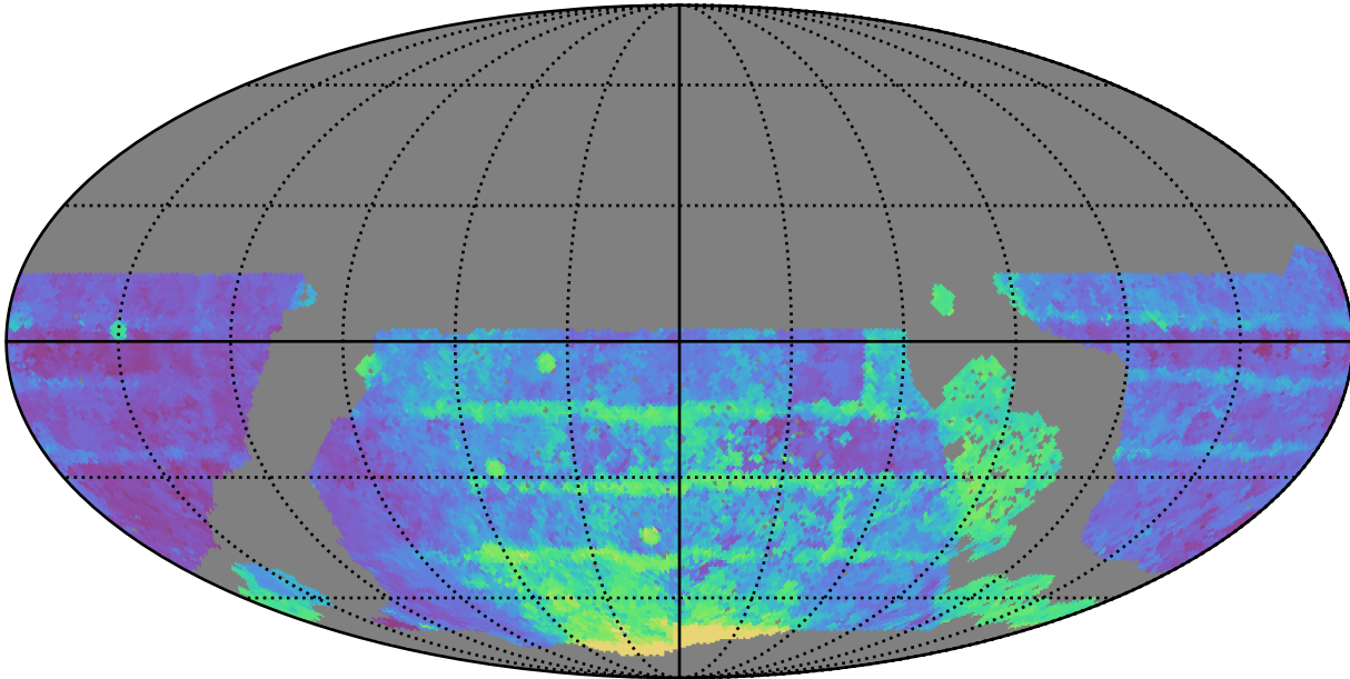
roll_uniform_early_half_accordion1_mjdp0_v3.4_10yrs WFD all bands: Median Season Length
