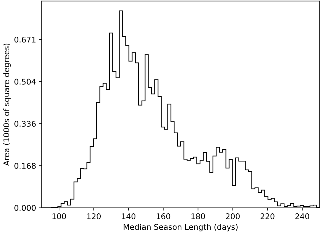
roll_uniform_early_half_accordion1_mjdp0_v3.4_10yrs WFD all bands: Median Season Length
