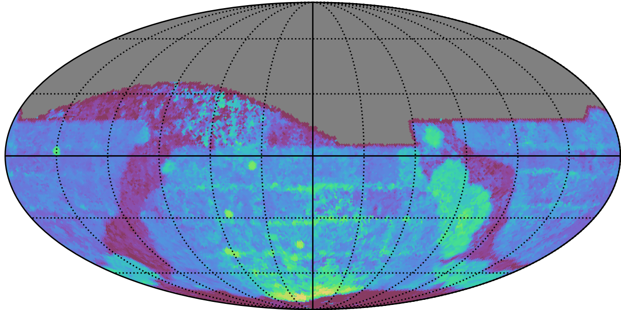
roll_uniform_early_half_accordion1_mjdp0_v3.4_10yrs All sky z band: Median Season Length
