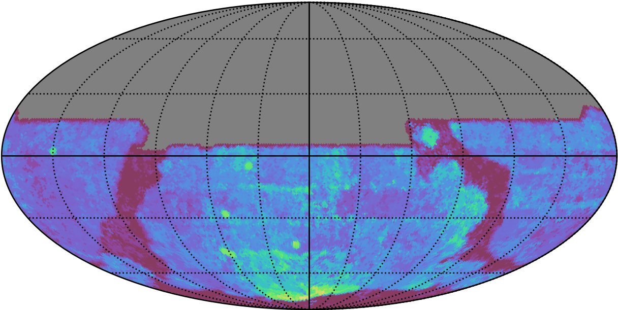
roll_uniform_early_half_accordion1_mjdp0_v3.4_10yrs All sky y band: Median Season Length
