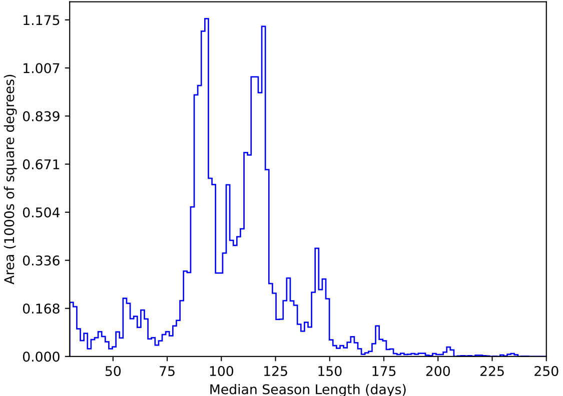
roll_uniform_early_half_accordion1_mjdp0_v3.4_10yrs All sky y band: Median Season Length
