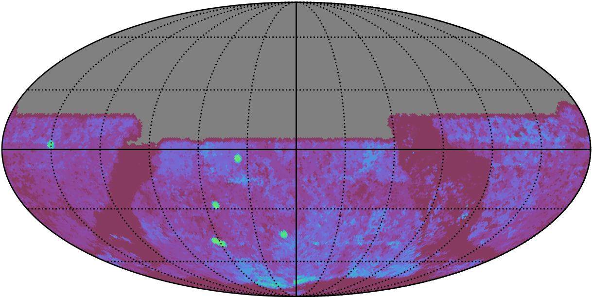
roll_uniform_early_half_accordion1_mjdp0_v3.4_10yrs All sky u band: Median Season Length
