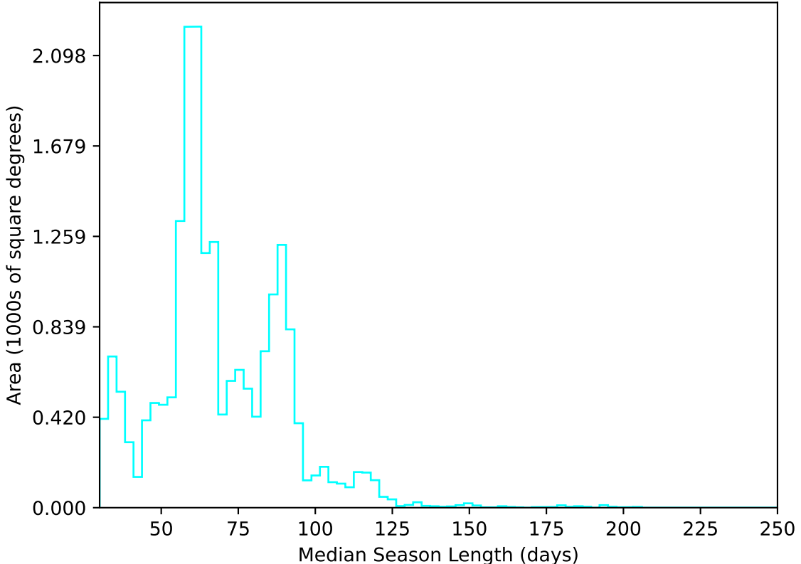
roll_uniform_early_half_accordion1_mjdp0_v3.4_10yrs All sky u band: Median Season Length
