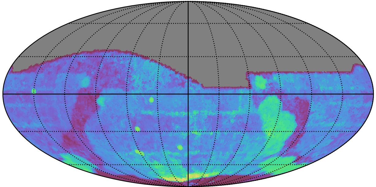
roll_uniform_early_half_accordion1_mjdp0_v3.4_10yrs All sky r band: Median Season Length
