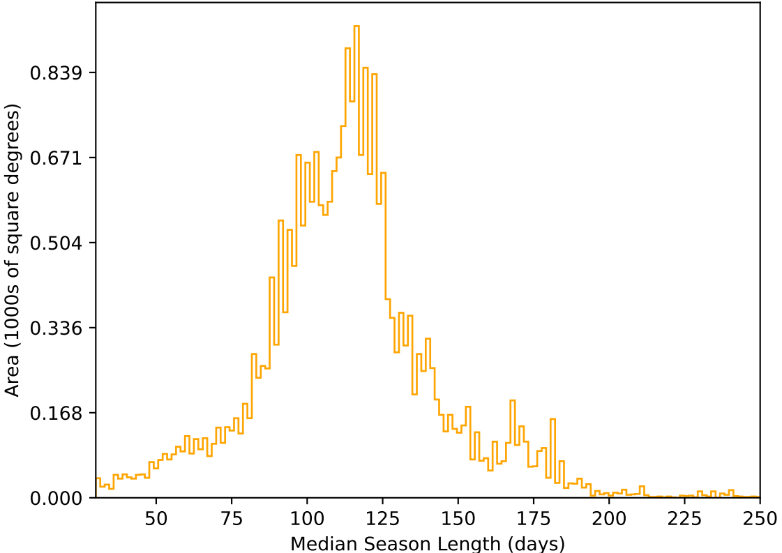
roll_uniform_early_half_accordion1_mjdp0_v3.4_10yrs All sky r band: Median Season Length
