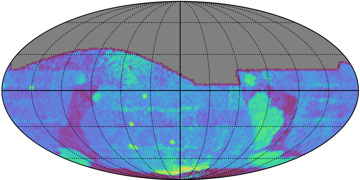
roll_uniform_early_half_accordion1_mjdp0_v3.4_10yrs All sky i band: Median Season Length
