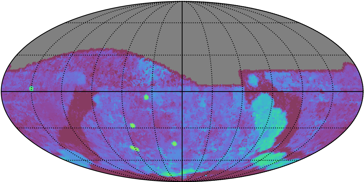
roll_uniform_early_half_accordion1_mjdp0_v3.4_10yrs All sky g band: Median Season Length
