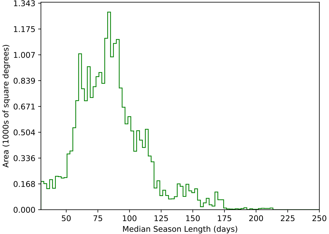
roll_uniform_early_half_accordion1_mjdp0_v3.4_10yrs All sky g band: Median Season Length
