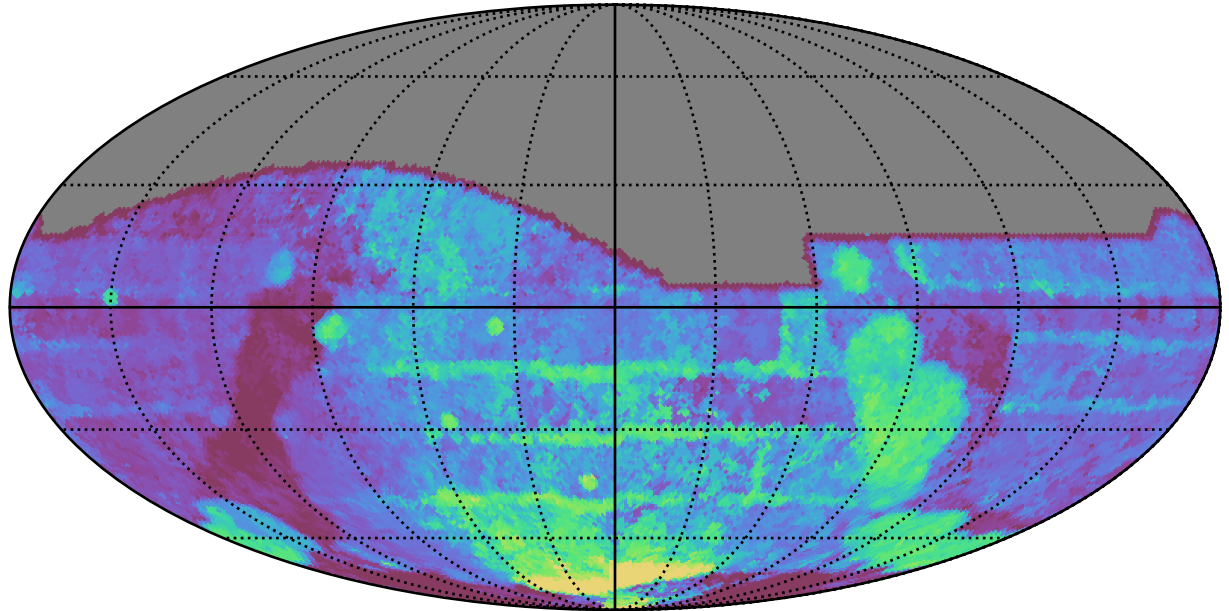
roll_uniform_early_half_accordion1_mjdp0_v3.4_10yrs All sky all bands: Median Season Length
