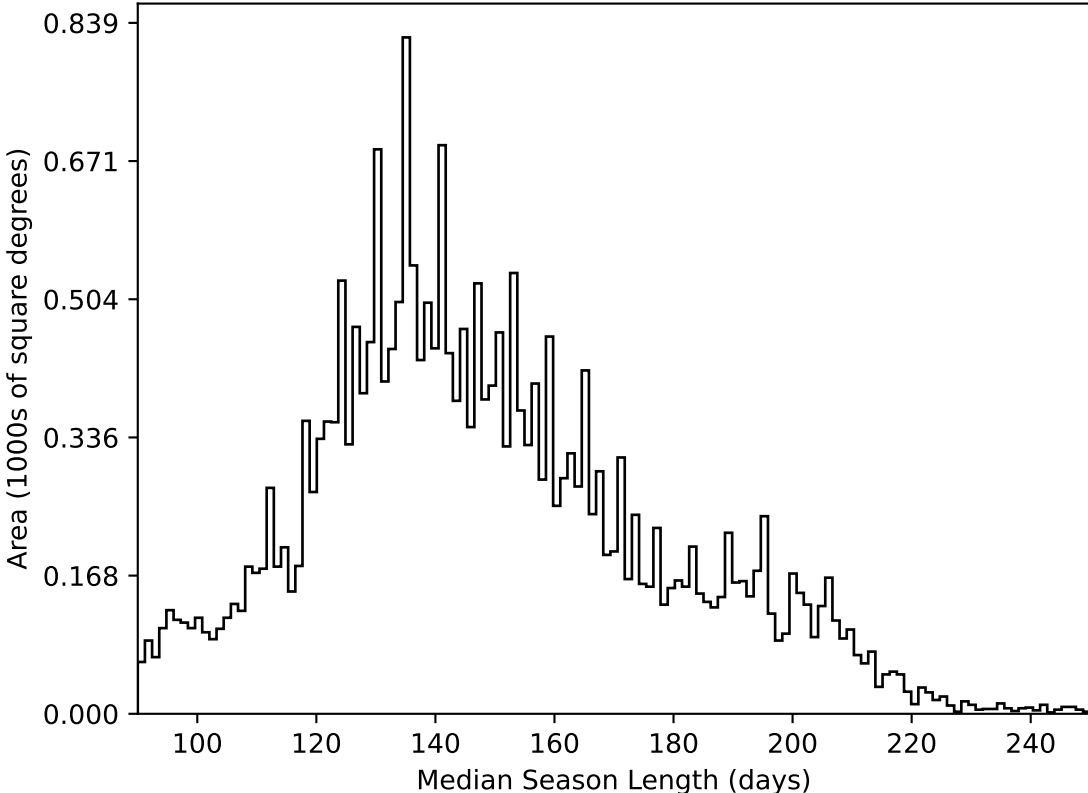
roll_uniform_early_half_accordion1_mjdp0_v3.4_10yrs All sky all bands: Median Season Length
