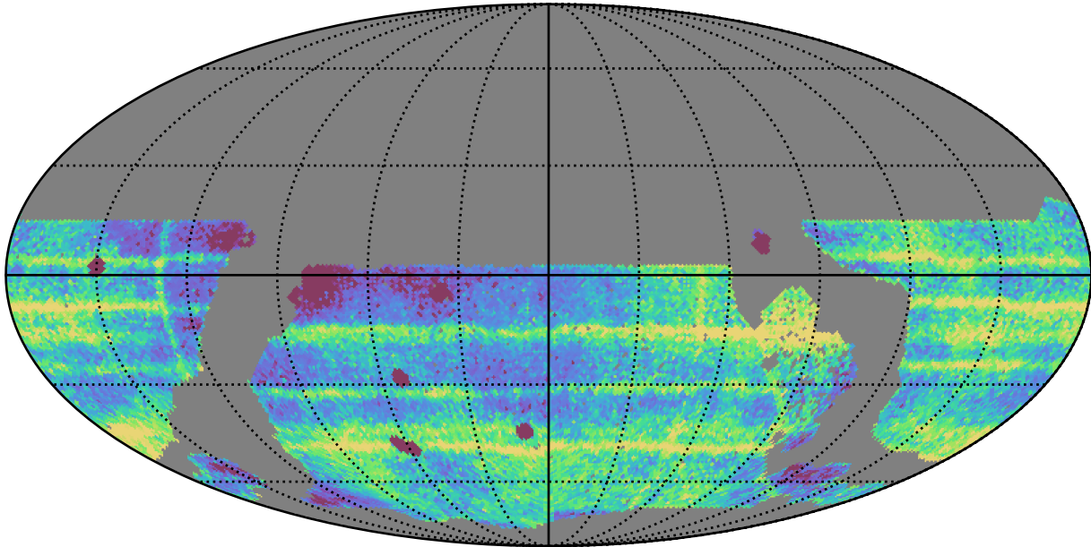
roll_uniform_early_half_accordion1_mjdp0_v3.4_10yrs WFD: Median Intra-Night Gap
