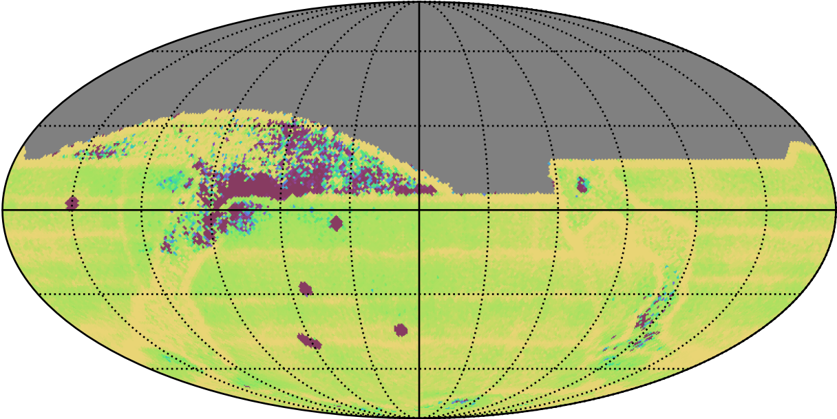
roll_uniform_early_half_accordion1_mjdp0_v3.4_10yrs All sky: Median Intra-Night Gap
