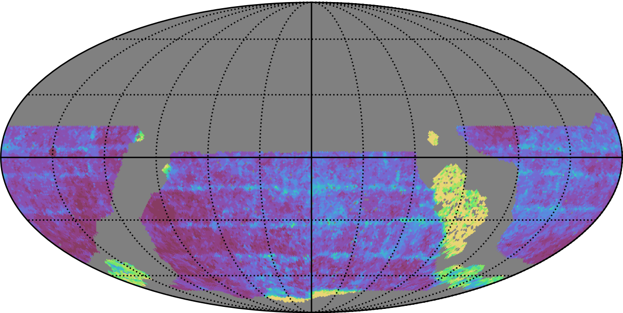
roll_uniform_early_half_accordion1_mjdp0_v3.4_10yrs WFD z band: Median Inter-Night Gap
