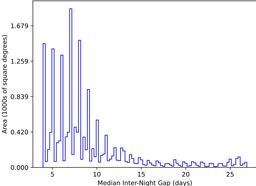
roll_uniform_early_half_accordion1_mjdp0_v3.4_10yrs WFD y band: Median Inter-Night Gap
