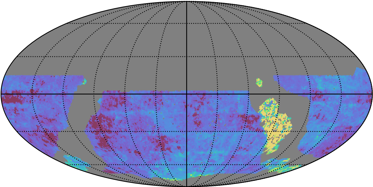
roll_uniform_early_half_accordion1_mjdp0_v3.4_10yrs WFD u band: Median Inter-Night Gap
