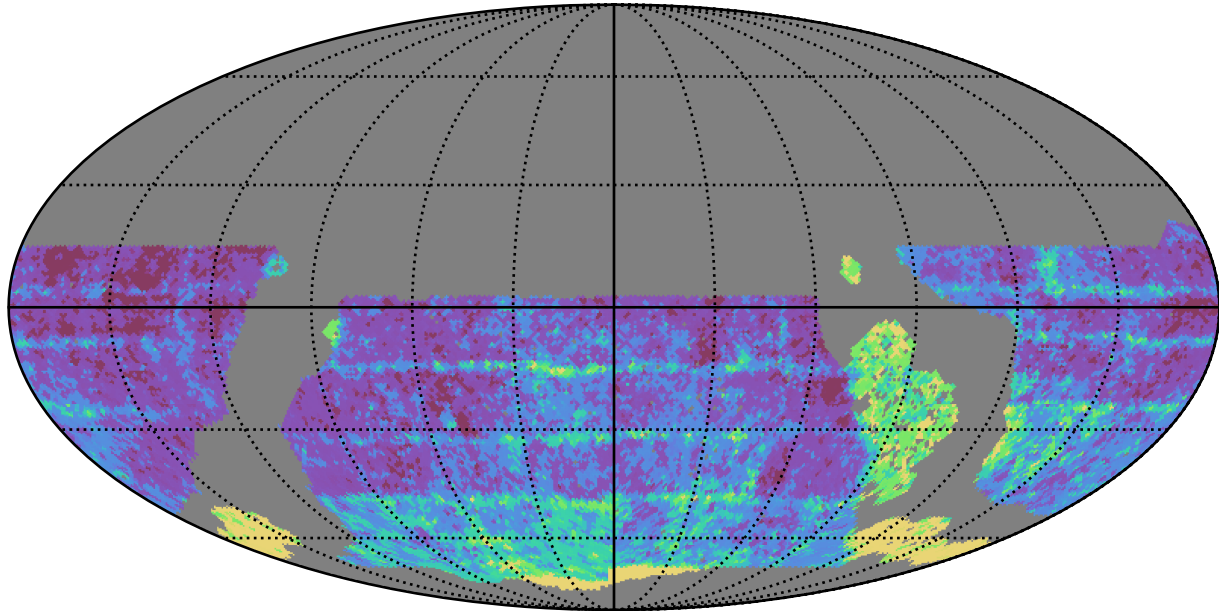
roll_uniform_early_half_accordion1_mjdp0_v3.4_10yrs WFD r band: Median Inter-Night Gap
