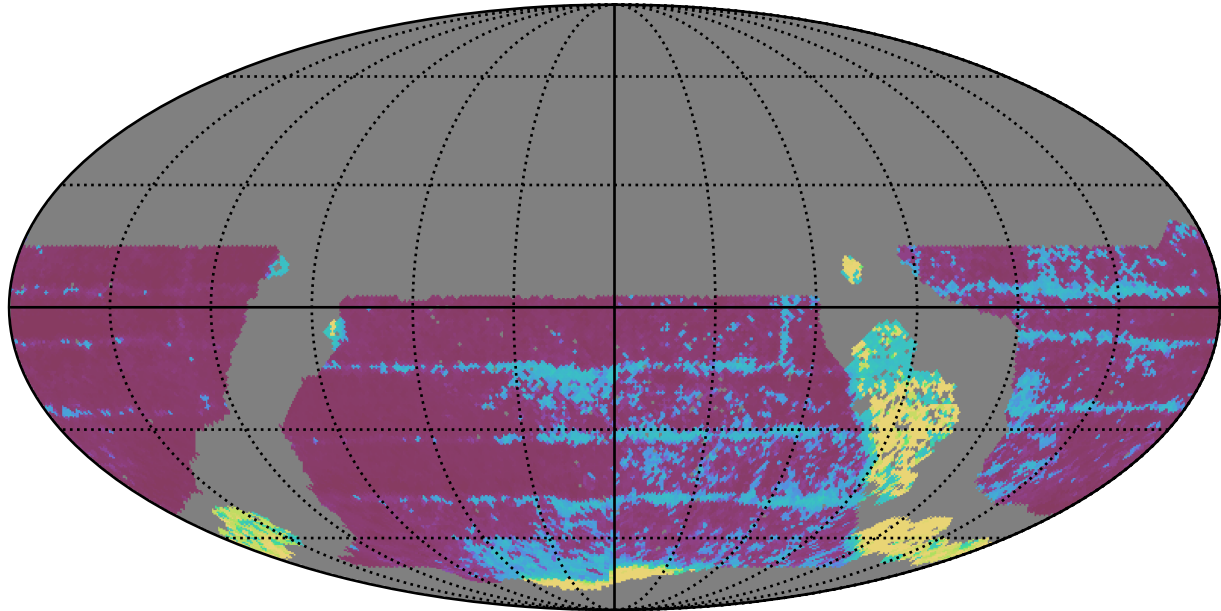
roll_uniform_early_half_accordion1_mjdp0_v3.4_10yrs WFD all bands: Median Inter-Night Gap
