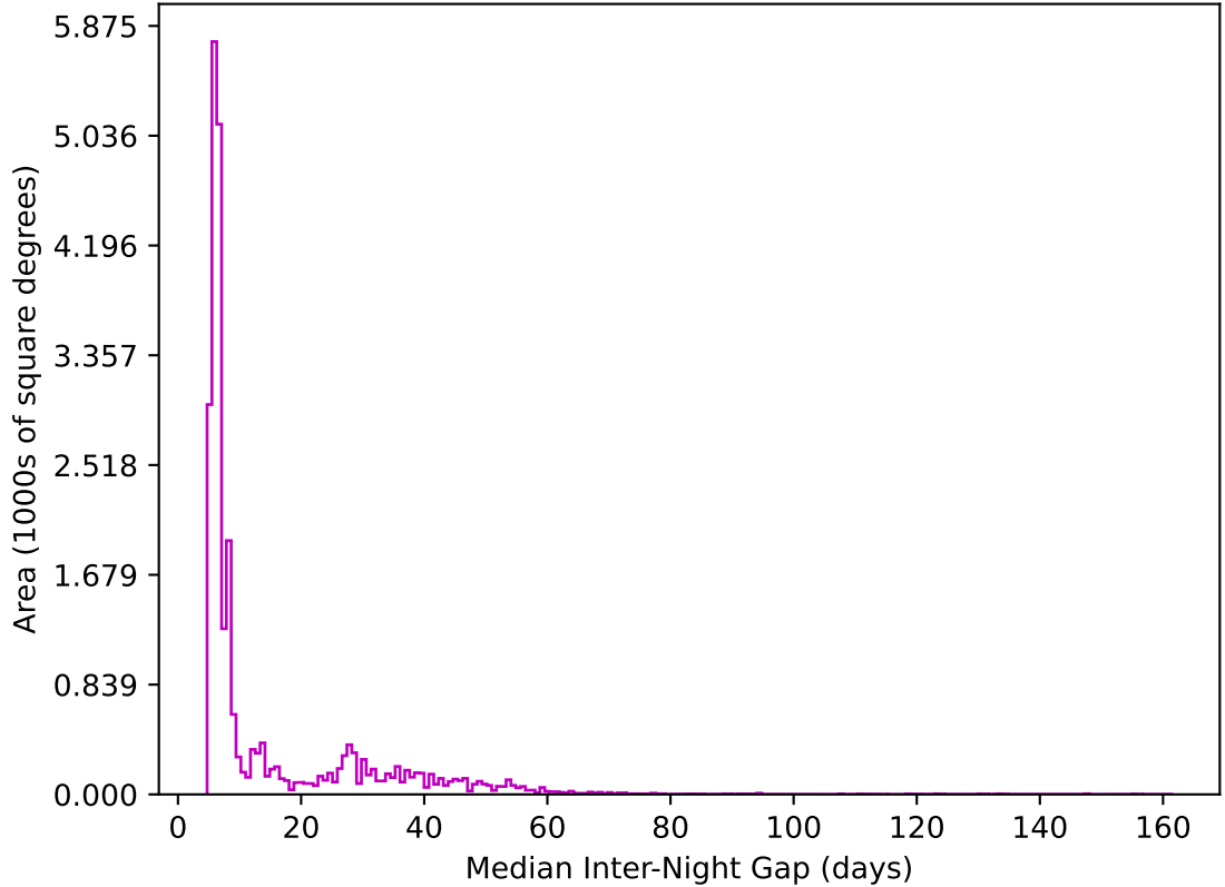
roll_uniform_early_half_accordion1_mjdp0_v3.4_10yrs All sky z band: Median Inter-Night Gap
