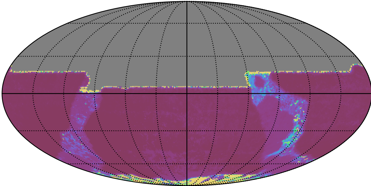
roll_uniform_early_half_accordion1_mjdp0_v3.4_10yrs All sky y band: Median Inter-Night Gap
