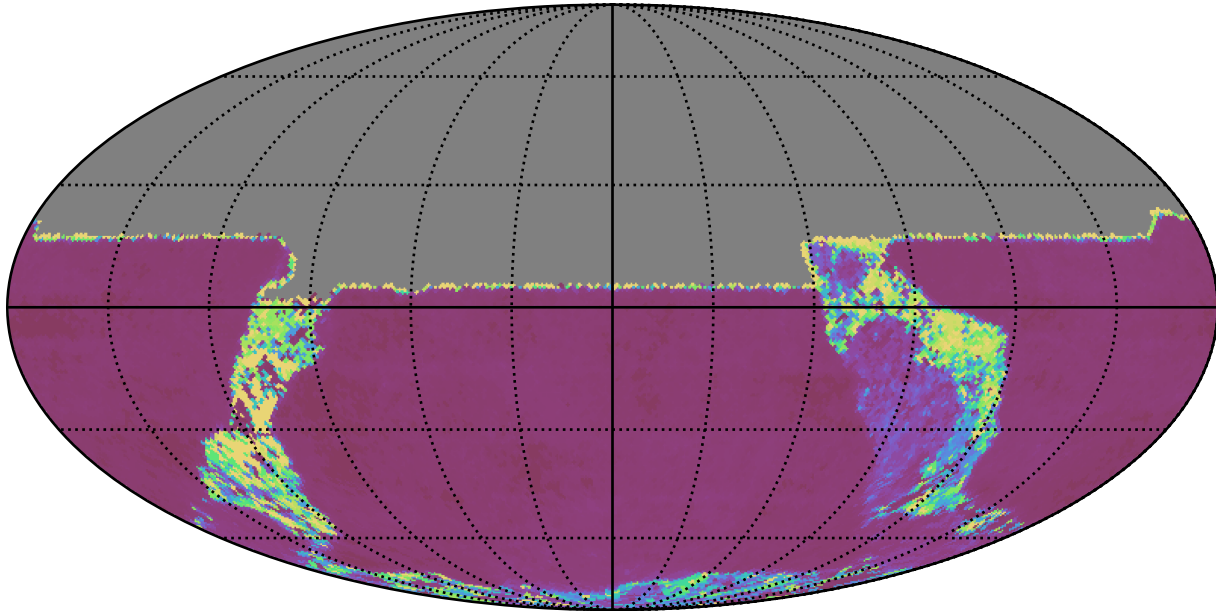
roll_uniform_early_half_accordion1_mjdp0_v3.4_10yrs All sky u band: Median Inter-Night Gap
