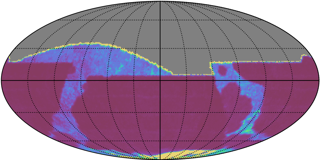
roll_uniform_early_half_accordion1_mjdp0_v3.4_10yrs All sky r band: Median Inter-Night Gap
