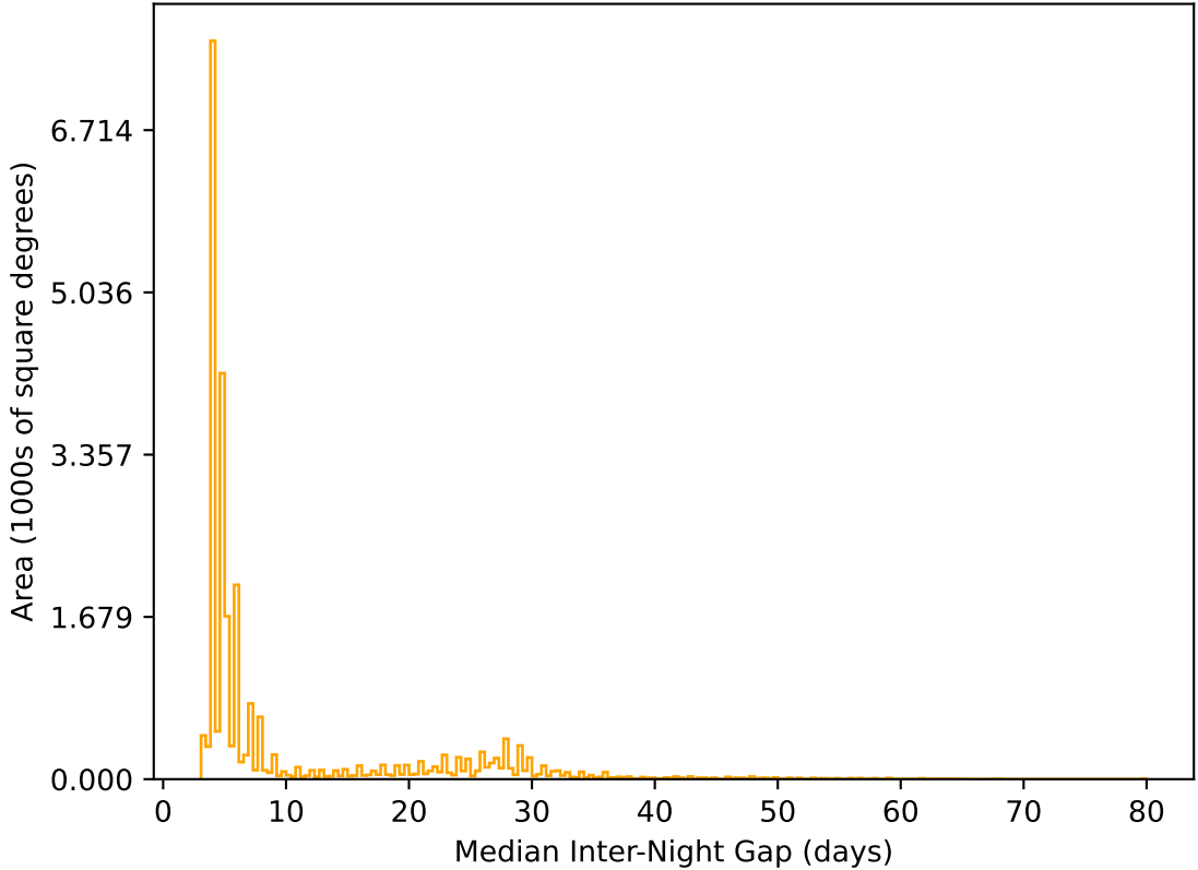
roll_uniform_early_half_accordion1_mjdp0_v3.4_10yrs All sky r band: Median Inter-Night Gap
