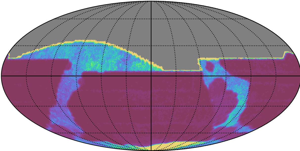
roll_uniform_early_half_accordion1_mjdp0_v3.4_10yrs All sky all bands: Median Inter-Night Gap
