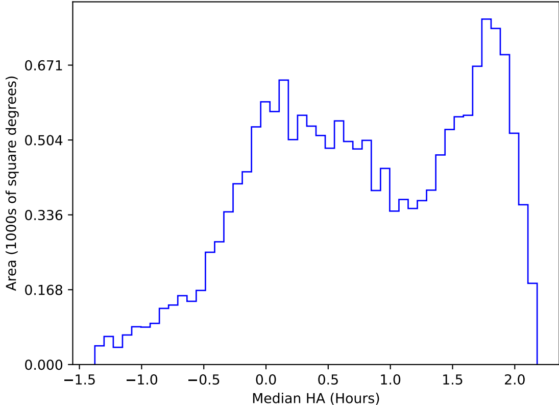
roll_uniform_early_half_accordion1_mjdp0_v3.4_10yrs WFD g band: Median HA
