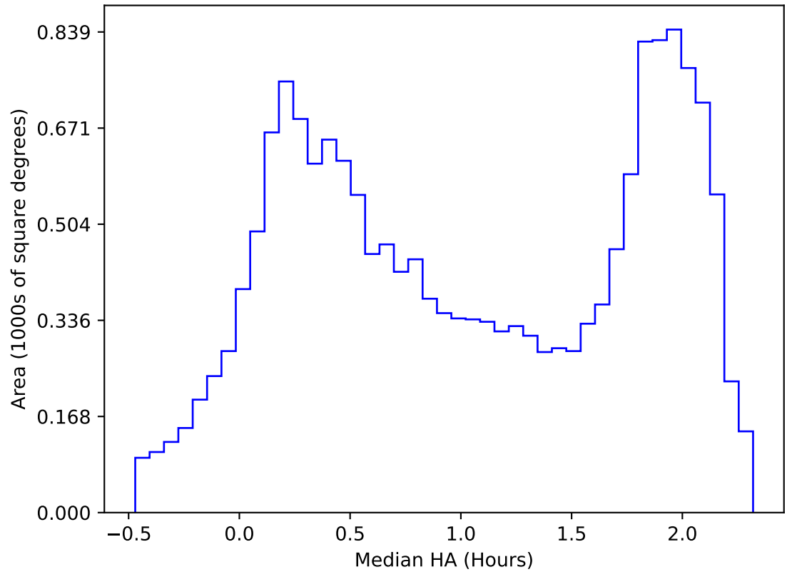
roll_uniform_early_half_accordion1_mjdp0_v3.4_10yrs WFD all bands: Median HA
