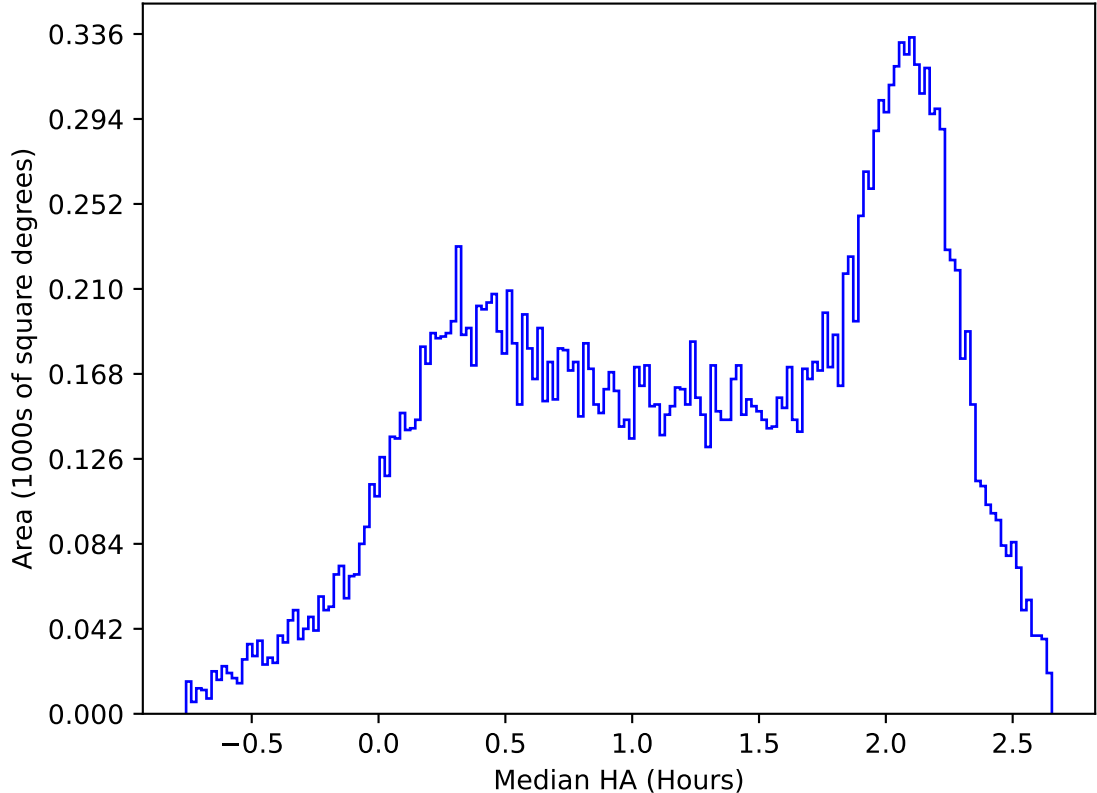
roll_uniform_early_half_accordion1_mjdp0_v3.4_10yrs All sky y band: Median HA
