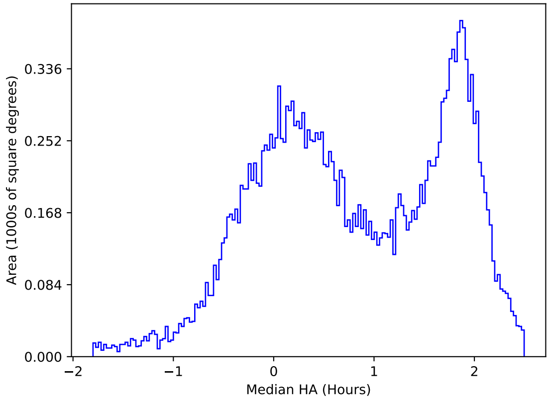
roll_uniform_early_half_accordion1_mjdp0_v3.4_10yrs All sky u band: Median HA
