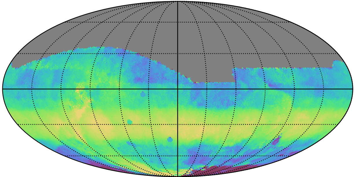
roll_uniform_early_half_accordion1_mjdp0_v3.4_10yrs All sky i band: Median HA
