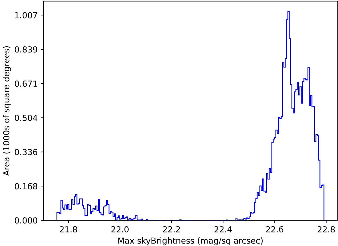
roll_uniform_early_half_accordion1_mjdp0_v3.4_10yrs Yr 1 all bands: Max skyBrightness
