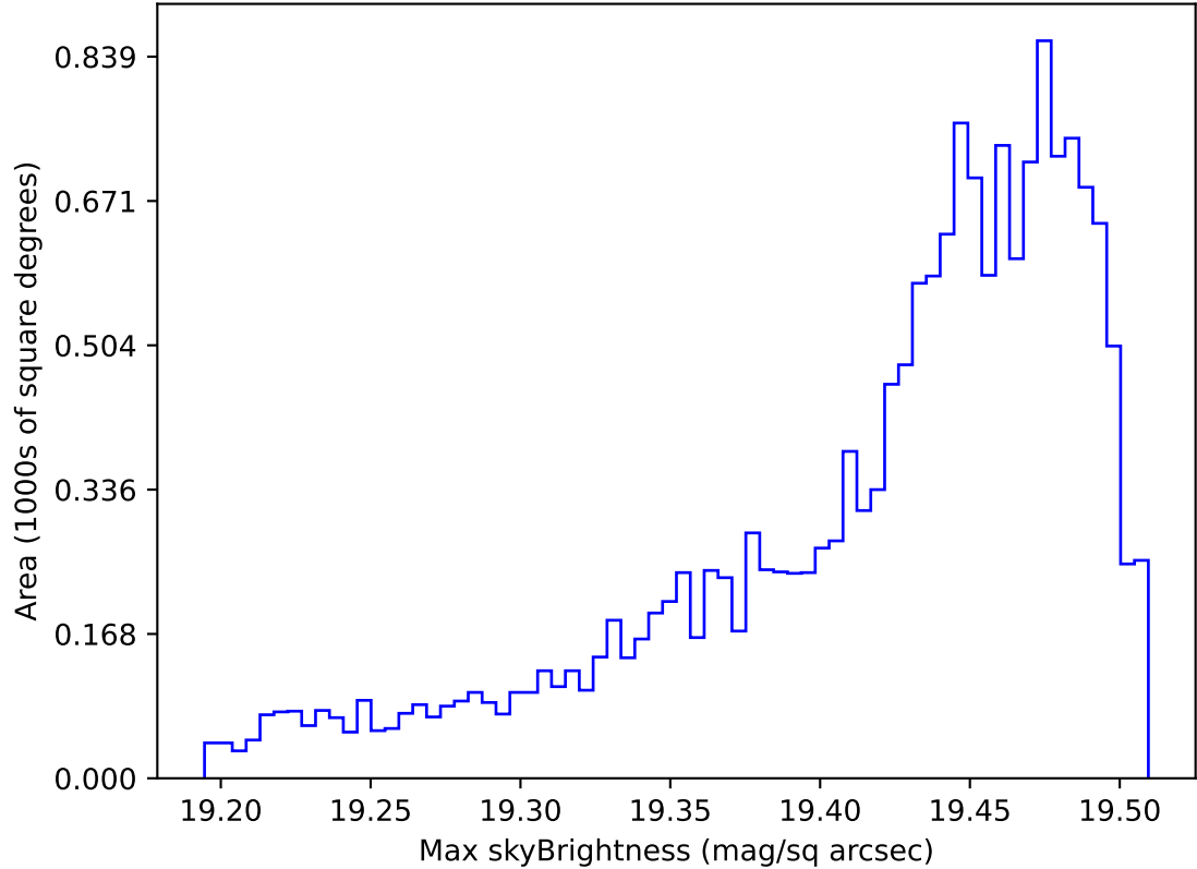
roll_uniform_early_half_accordion1_mjdp0_v3.4_10yrs WFD z band: Max skyBrightness
