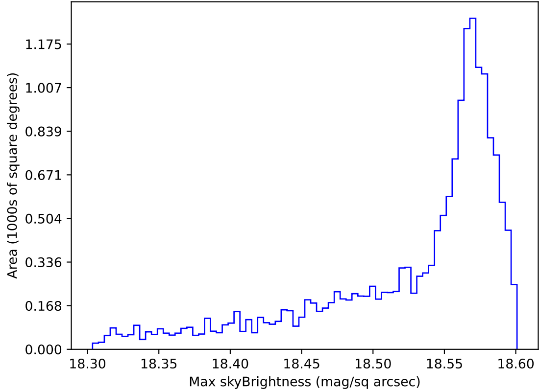
roll_uniform_early_half_accordion1_mjdp0_v3.4_10yrs WFD y band: Max skyBrightness
