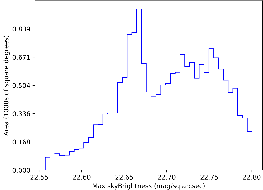
roll_uniform_early_half_accordion1_mjdp0_v3.4_10yrs WFD u band: Max skyBrightness
