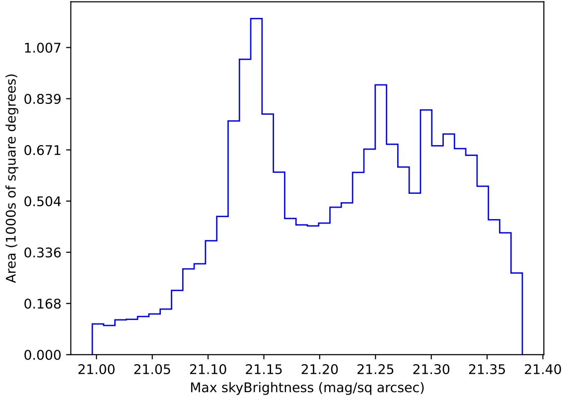
roll_uniform_early_half_accordion1_mjdp0_v3.4_10yrs WFD r band: Max skyBrightness
