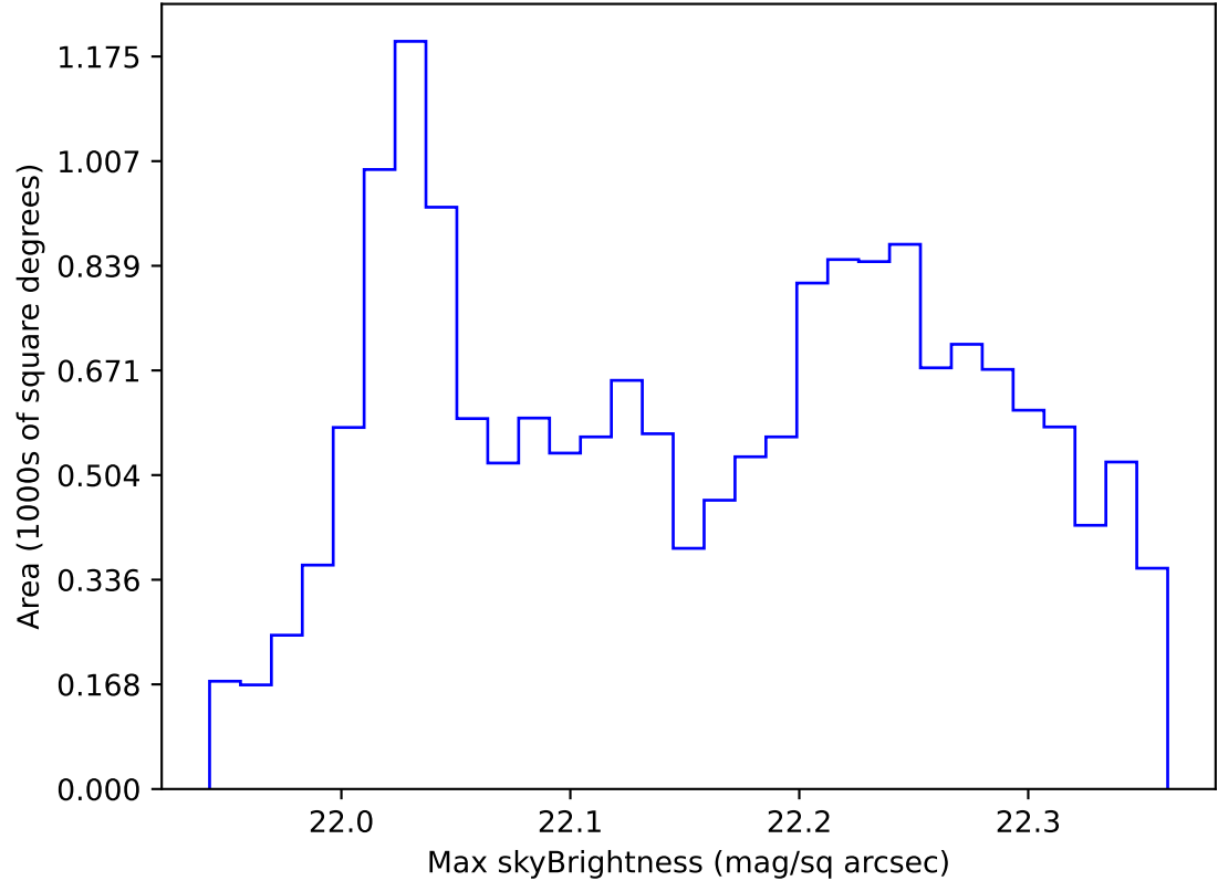
roll_uniform_early_half_accordion1_mjdp0_v3.4_10yrs WFD g band: Max skyBrightness
