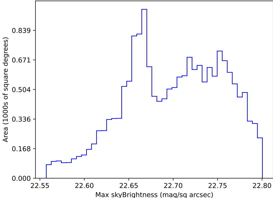
roll_uniform_early_half_accordion1_mjdp0_v3.4_10yrs WFD all bands: Max skyBrightness
