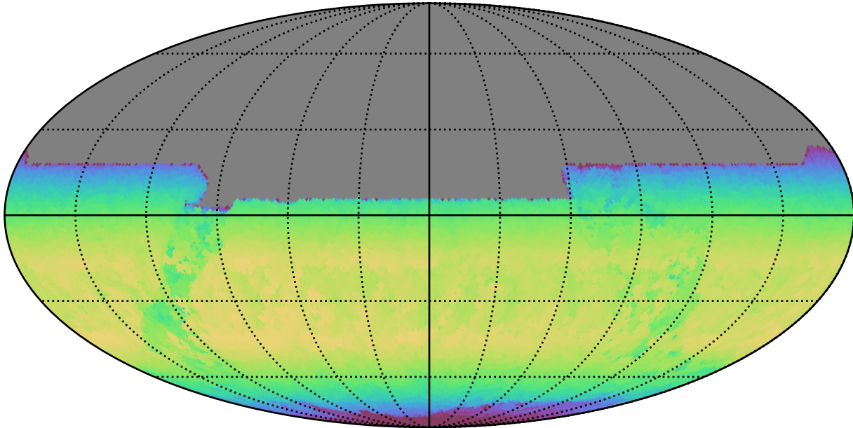
roll_uniform_early_half_accordion1_mjdp0_v3.4_10yrs All sky y band: Max skyBrightness
