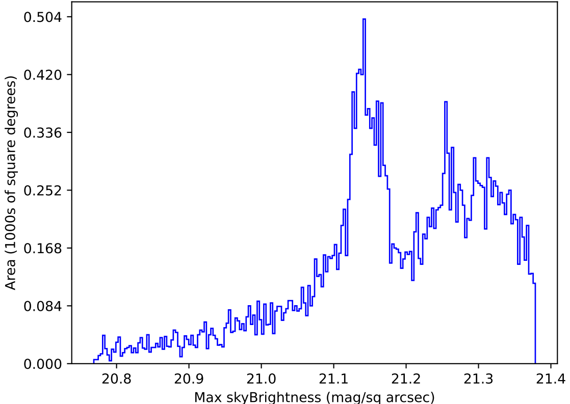
roll_uniform_early_half_accordion1_mjdp0_v3.4_10yrs All sky r band: Max skyBrightness
