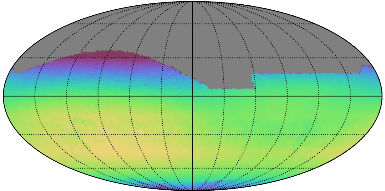
roll_uniform_early_half_accordion1_mjdp0_v3.4_10yrs All sky i band: Max skyBrightness
