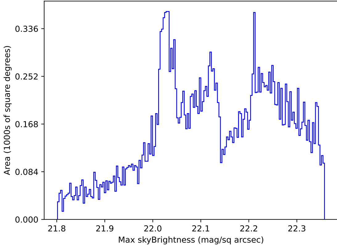
roll_uniform_early_half_accordion1_mjdp0_v3.4_10yrs All sky g band: Max skyBrightness
