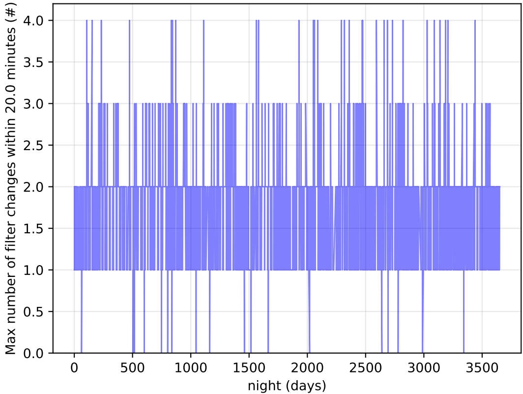
roll_uniform_early_half_accordion1_mjdp0_v3.4_10yrs Per Night: Max number of filter changes within 20.0 minutes
